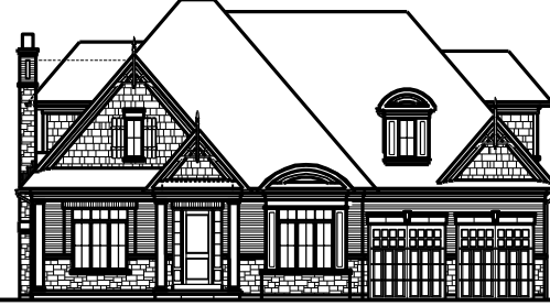
C5BUN 02 FRONT ELEVATION 'B'
